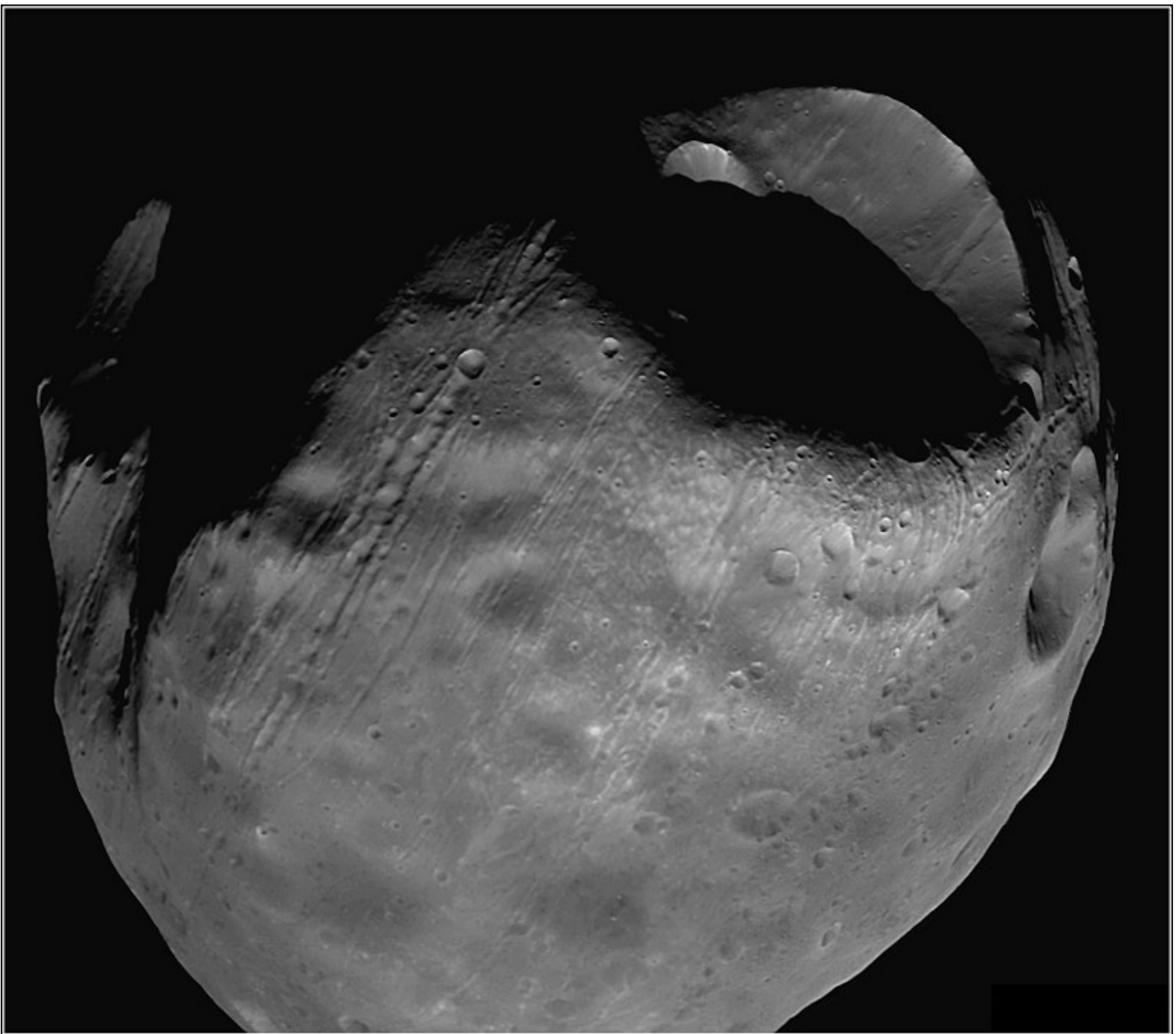
Phobos
